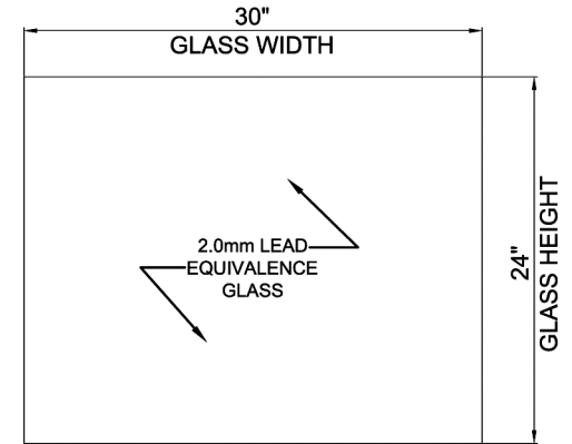
(B) 1 GLASS ELEVATION
