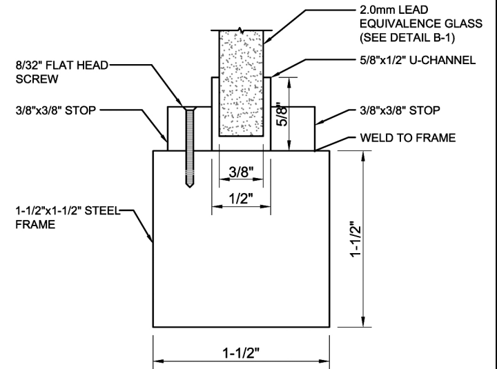
(C) 1 SECTION AT FRAME
